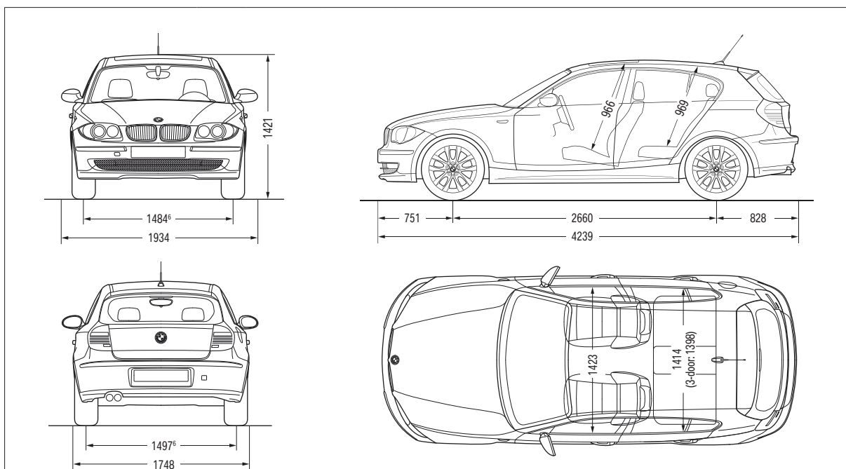
All dimensions in millimetres (shown here the BMW 1 Series 5-door). Luggage compartment capacity (measured according to VDA standard) approx. 330 to 1,150 litres (11.7 to 40.6 cu ft).
